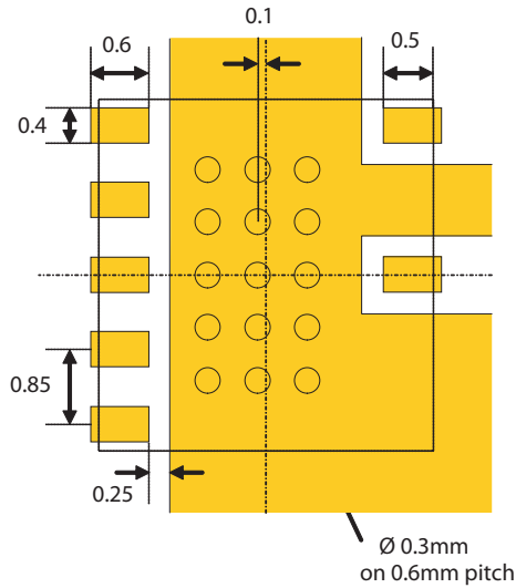
Figure 15. Metallization
